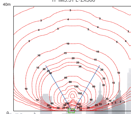
ISOLUX DIAGRAMS TF IM5.5Y L-2X300
