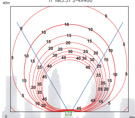
ISOLUX DIAGRAMS TF IM5.5Y J-4X400
