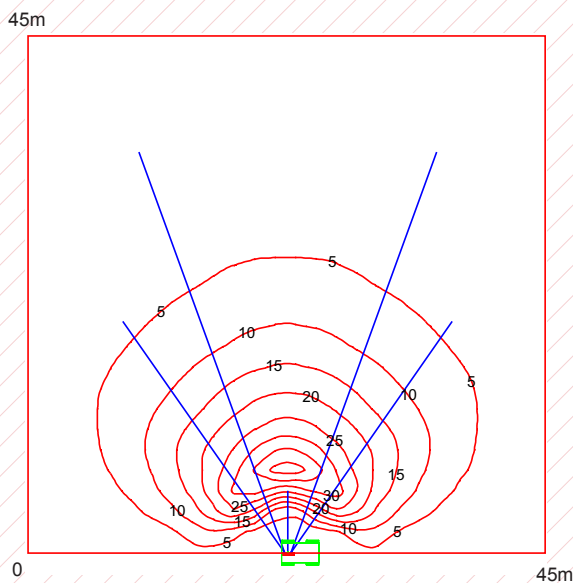
ILLUMINATED AREA 750Mq ISOLUX DIAGRAMS
